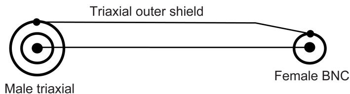
Figure 2: Model 7078-TRX-GND schematic
